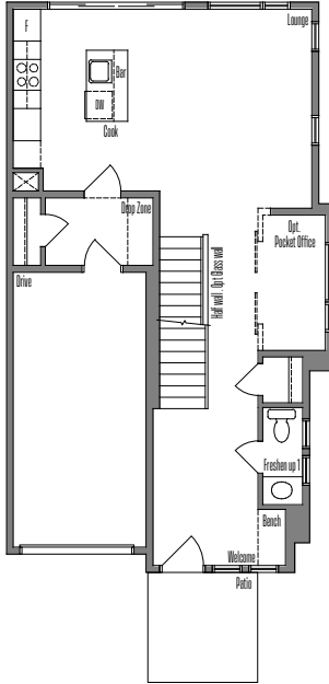
MAIN FLOOR PLAN #152
