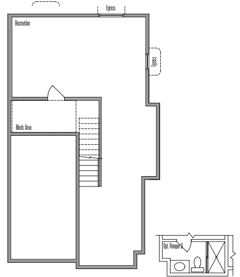
BASEMENT PLAN #152
