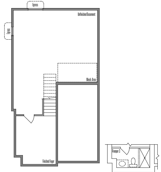
BASEMENT PLAN #138
